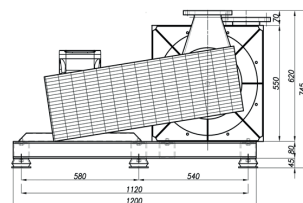
MULTISTAGE CENTRIFUGAL BLOWER multistage centrifugal blower 4,500 m³/h, 9,500 mmAq
