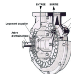
PERIPHERAL TOROIDAL CHANEL BLOWER max capacity 1,900 m 3 /h, 8,000 mmAq
