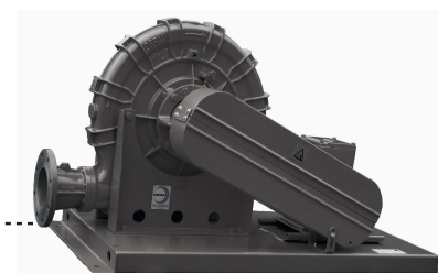
ALUMINIUM CASTING CENTRIFUGAL BLOWER max capacity 2,800 m³/h, 1,700 mmAq
