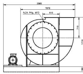
CENTRIFUGAL BLOWER centrifugal fans 800,000 m 3 /h, 2,500 mmAq
