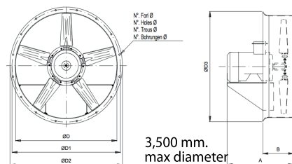
AXIAL FANS | SPMD & SPMDR axial fans 1,000,000 m³/h, 250 mmAq
